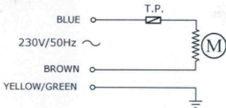
Wiring diagram
